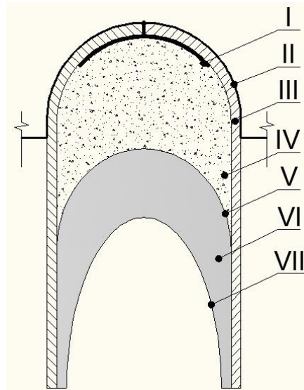
Figure 3 – Charge design.
