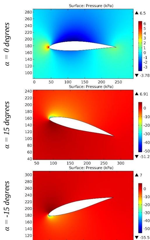
Figure 58. The pressure contours on the surfaces of the NA63A414 airfoil.
