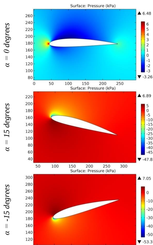
Figure 114. The pressure contours on the surfaces of the NACA 2412 airfoil.
