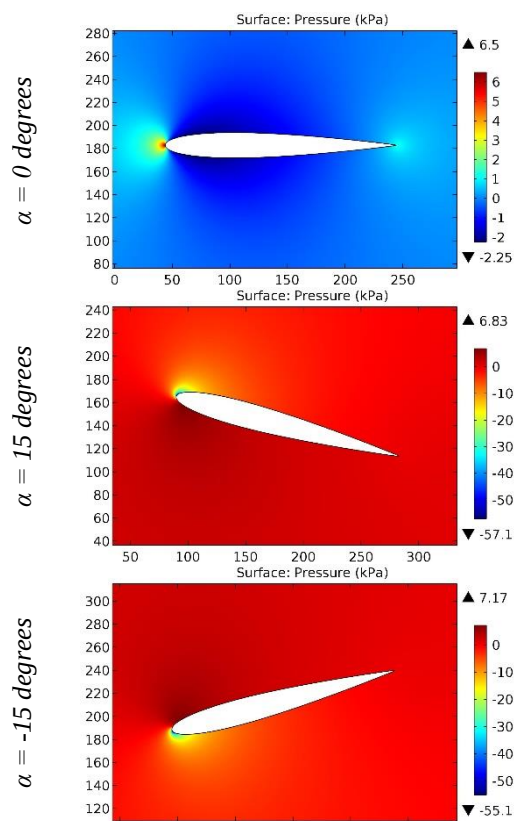
Figure 84. The pressure contours on the surfaces of the NACA 0011 airfoil.
