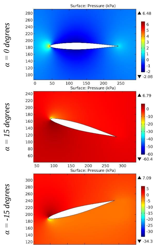
Figure 72. The pressure contours on the surfaces of the NA64A010 airfoil.
