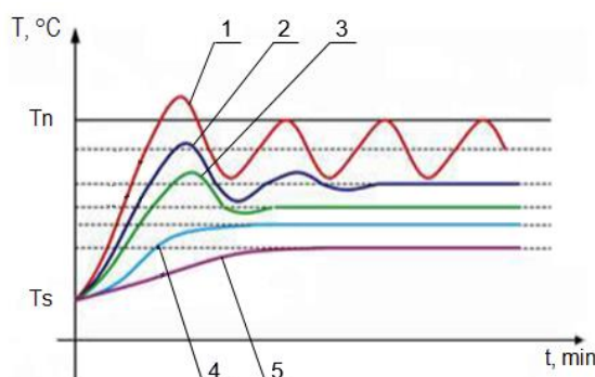
Fig 5. Illustration of the influence of PID coefficients on the curve shape
