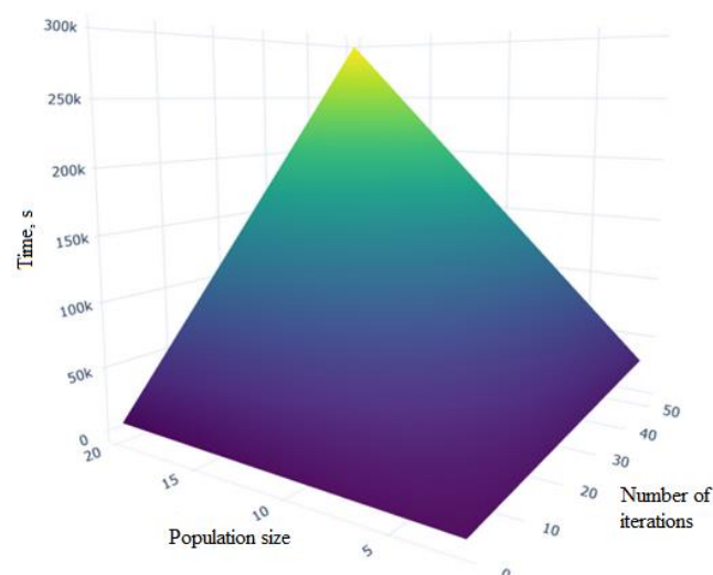
Fig.13 Genetic-algorithm run-time
