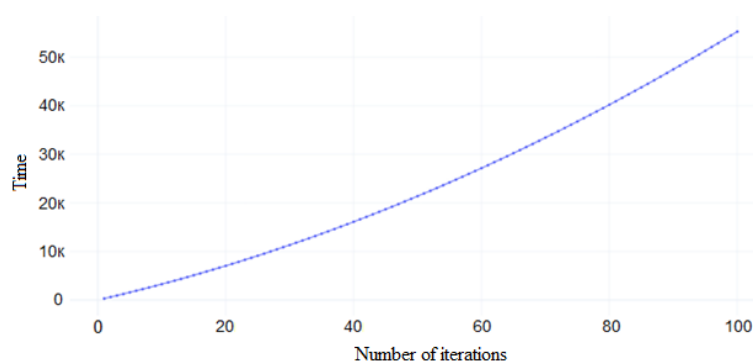
Fig.14 Bayesian-optimisation run-time
