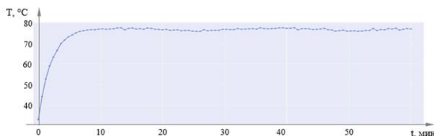
Fig.19 CPU-temperature curve after PID tuning
