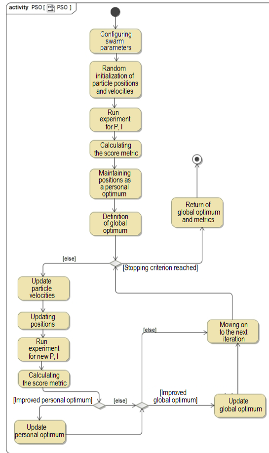
Fig.6 Block diagram of the particle-swarm optimisation algorithm
