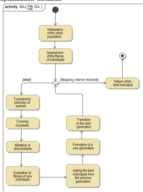
Fig.9 Genetic Algorithm flowchart
