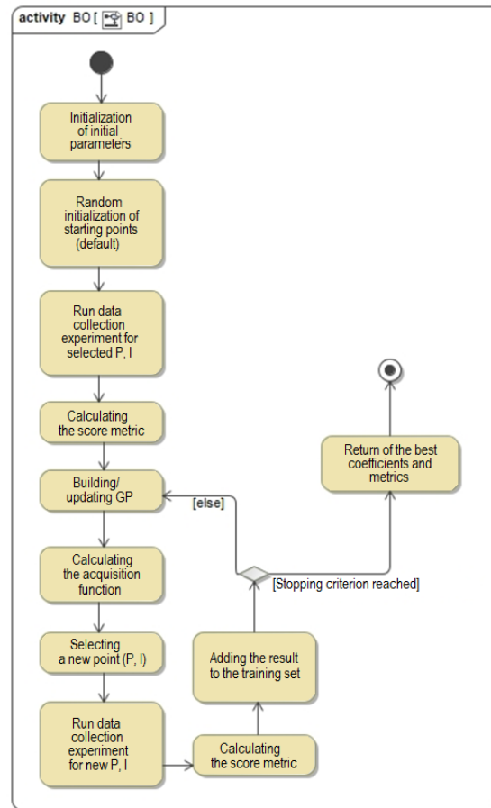
Fig.8 Block diagram of the Bayesian-optimisation procedure
