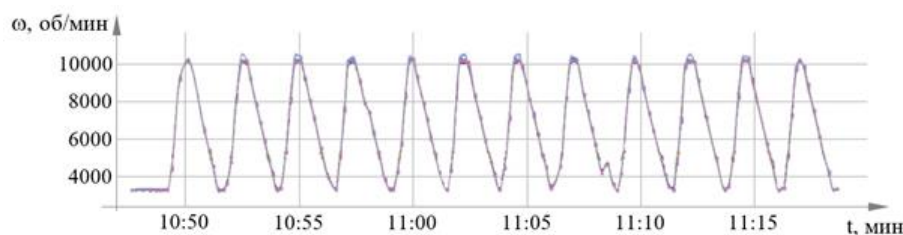
Fig.16 Fan-speed curve before PID tuning
