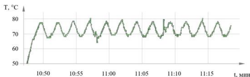
Fig.18 CPU-temperature curve before PID tuning
