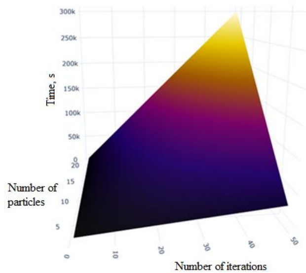
Fig.11 PSO run-time versus iteration count and particle number
