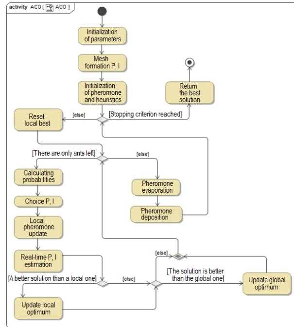
Fig.7 Block diagram of the ant-colony algorithm
