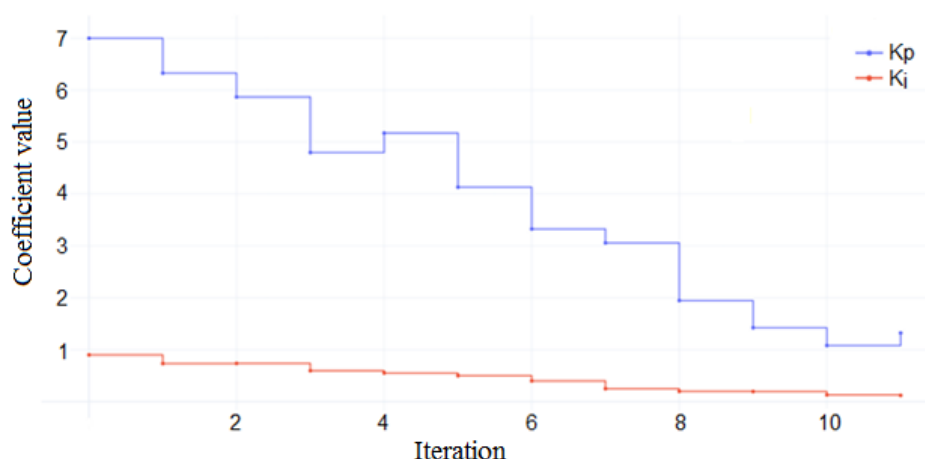
Fig.10 Evolution of PID coefficients during Bayesian optimization
